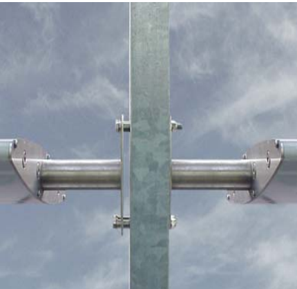
Parallel offset fixing bracket. A detailed view of a 90° parallel off-set fixing bracket attaching a csairfoil AF 270F blade onto a vertical support segment is illustrated above. The brackets are screwed directly onto the end of the blade thanks to the special screw channels incorporated into the extrusion. The bracket-blade unit is then fixed with bolts onto the support segment. The availability of parallel off-set fixing brackets and compound angle fixing brackets in a wide variety of angles cater for an unlimited range of design possibilities and adapt to virtually any project specifications.
