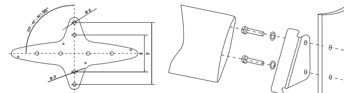
Insertion fixing plate (only AF 100) made of stainless steel is simply inserted into the blade and fixed with screws onto the structural support. Available in any desired angle.
