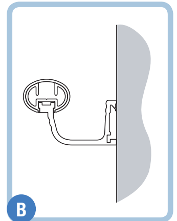
Tubular handrail HR 06
