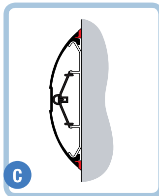
Smooth Crash rail Aronde 170 Duo
