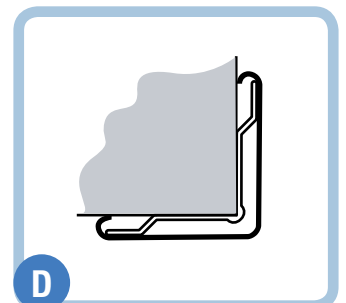
Surface Mounted Corner guard SSM 20 C/S Acrovyn® Faux Brushed Silver
