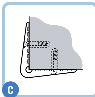
C/S Stelatex® Rubber Corner guard 100 C
