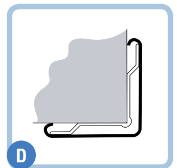
Surface Mounted Corner guard SSM 20 C/S Acrovyn® Faux Wood
