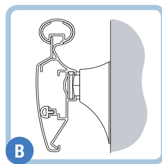
Handrail/Bumper guard HRB 20 Duo
