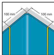
Radiused internal angle thermoformed
