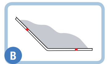
C/S Acrovyn® sheet Thermoformed external angle 135° with welded joint to the adjacent sheet
