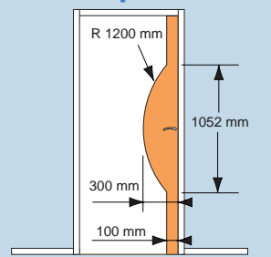
RAINBOW with strip
