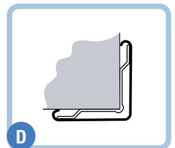
Surface Mounted Corner guard SSM 20
