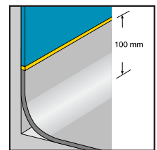
Heat-sealed junction with flexible flooring
